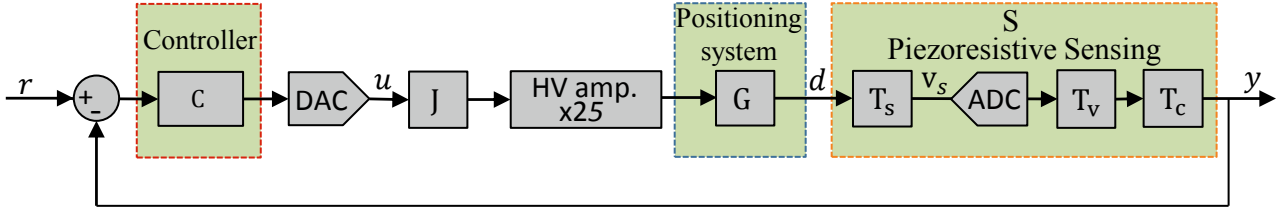
Fig. 7. The block diagram of the control law.
