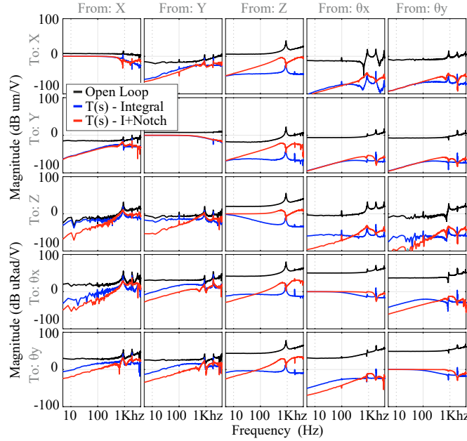
Fig. 8. The open-loop and closed-loop frequency responses.
