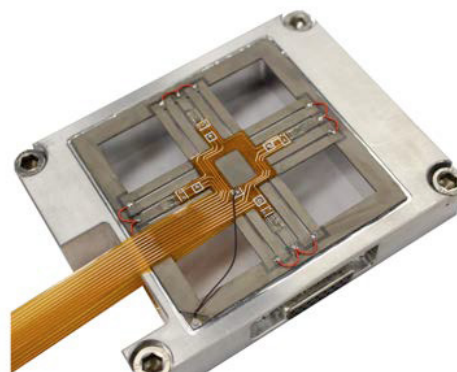
Fig. 1. Monolithic bimorph nanopositioner mounted on a base.
