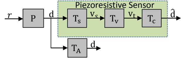
Fig. 5. The signal processing chain of the sensor calibration. \mathbf{P} is the nanopositioner, \mathbf{T}_s is the sensor matrix, \mathbf{T}_v is the thermal stability matrix, \mathbf{T}_c is the calibration matrix and \mathbf{T}_A is the calibration sensor.
