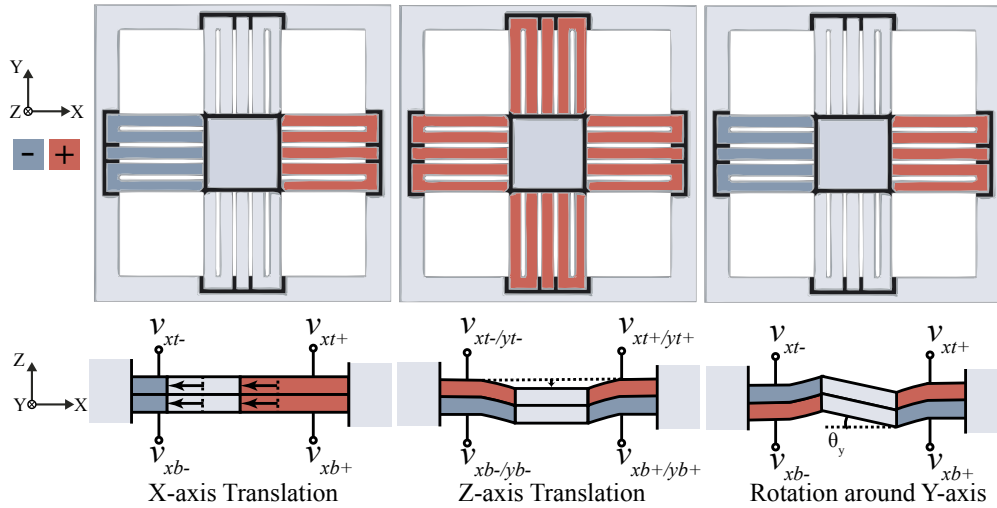
Fig. 2. The five-axis motions generated with different applied voltages.
