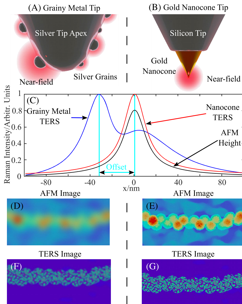
FIGURE 1 An illustrative comparison of a grainy silver probe where a grain has not formed at the tip apex (A) and a gold nanocone probe (B). The electric field distribution under each probe was calculated using boundary element method simulations plotted in (C). 20 The grainy probe has multiple hotspots, resulting in two enhancement peaks that will introduce artefacts into TERS maps. Furthermore, there is an offset between the AFM height and TERS measurements. Finally, the increased tip diameter results in decreased AFM and TERS image resolution shown in (D) and (F), respectively. The nanocone probe circumvents these issues as the physical tip apex functions as a single enhancement site with a small diameter, resulting in artefact-free, high-resolution and collocated AFM and TERS images as shown in (E) and (G).
